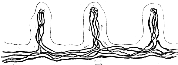
Diagram of three papillae from the frog's tongue, to show the arrangement of the nerve fibres.
